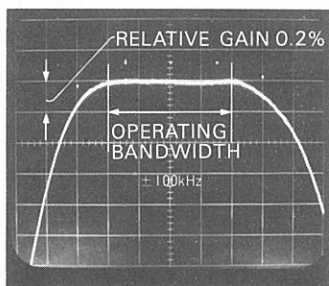
Fig.2 Differential Gain Characteristics of the Discriminator.
