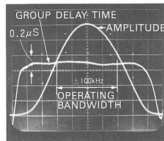
Fig. 1 Group Delay Time and Amplitude Characteristics of the IF circuitry.
